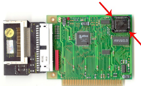
ROM Location and Pry Removal
