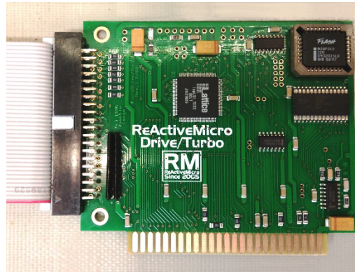
IDE Connected Properly
